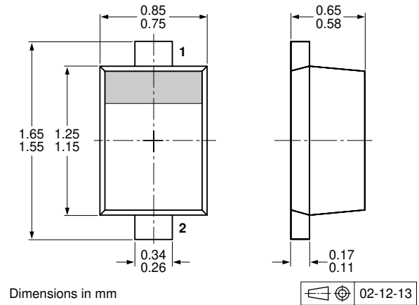
Fig 8. Package outline PESD3V3L1UB (SOD523/SC-79)
