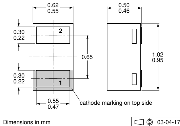
Fig 9. Package outline PESD3V3L1UL (SOD882)
