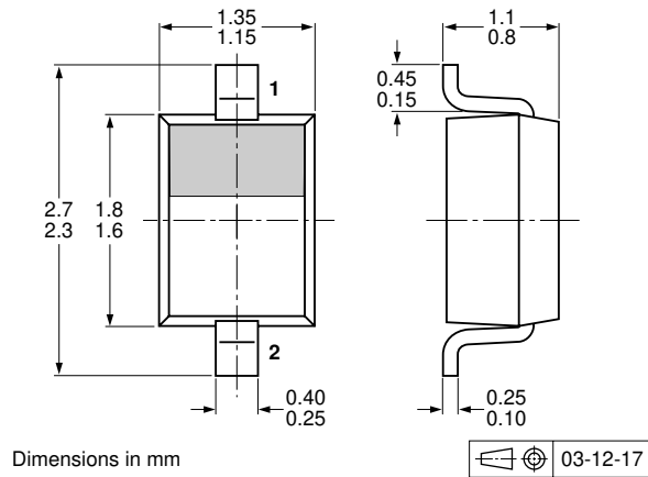
Fig 7. Package outline PESD3V3L1UA (SOD323/SC-76)
