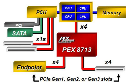
Figure 6. Host Centric Dual Upstream
