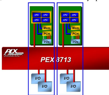
Figure 7. Multi-Host System
