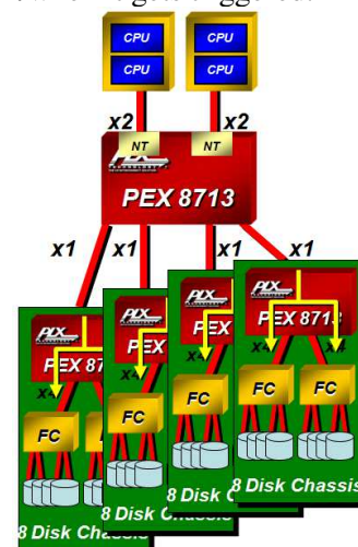
Figure 9. N+1 Failover
