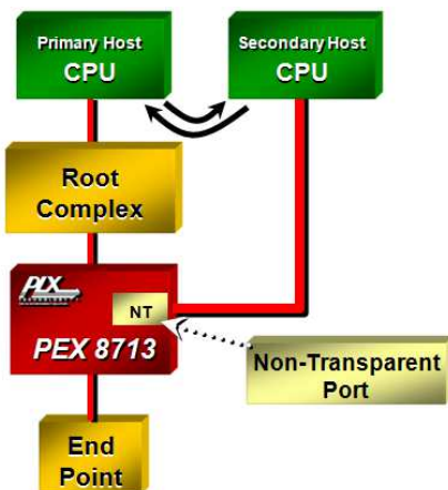
Figure 3. Non-Transparent Port
