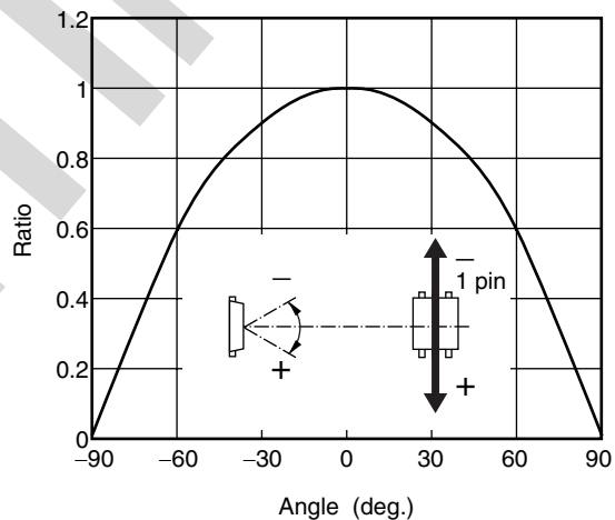
DIRECTIONAL CHARACTERISTICS 2
