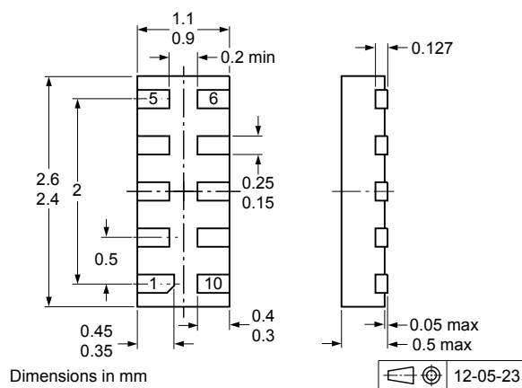
Fig. 13. Package outline DFN2510A-10 (SOT1176-1)
