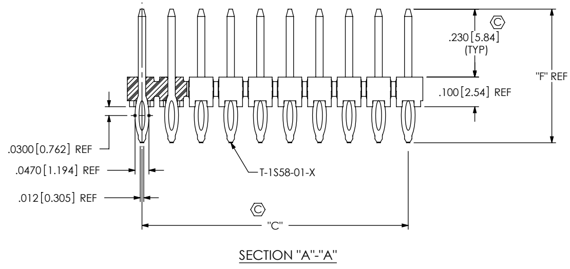
FIG 1 (PHT-1XX-01-X-3 SHOWN)
