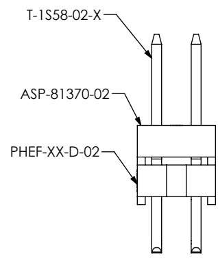
SECTION "H"-"H"
