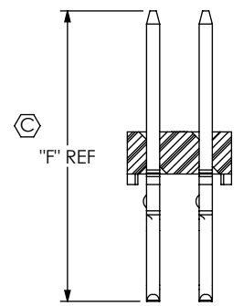
IN-PROGRESS -D ROW (FOR -02, -03 & -04 LEAD STYLE ONLY)
