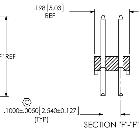
FIG 3 (PHT-1XX-01-X-D SHOWN) (SAME AS FIG 1, EXCEPT AS SHOWN)
