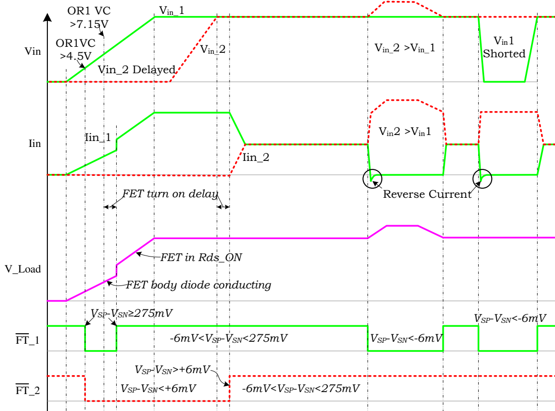
Figure 6: PI2126 Timing Diagram
