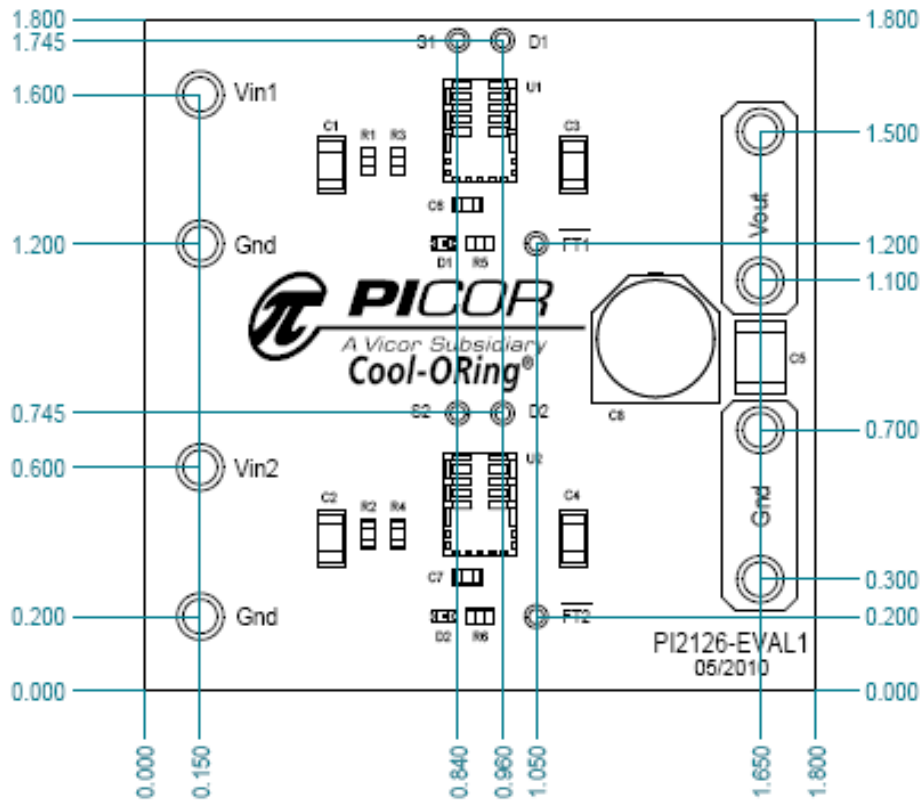
Figure 9: PI2126-EVAL1 evaluation board mechanical drawing.
