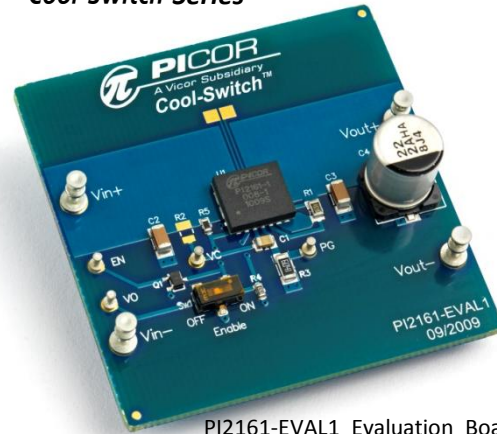
PI2161-EVAL1 Evaluation Board featuring the Cool-Switch PI2161 Full-Function Load Disconnect Switch.
