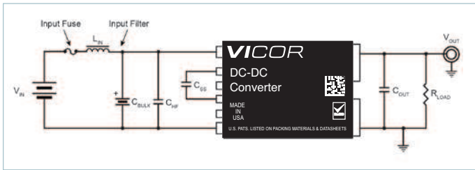
Figure 41 — PI31xx-00-HVMZ Shown With System Fuse, Filter, Decoupling And Extended Soft Start
