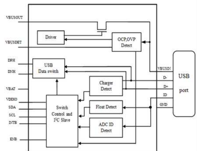
Figure 1. PI3USB9281C Block diagram
