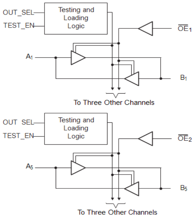
Figure 1: Block Diagram
