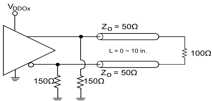
LVPECL Buffer
