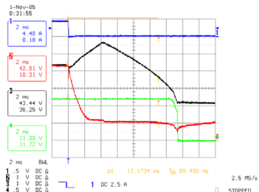
Figure 8. Holdup Performance; Loss of Feed A (with Feed B=0Vdc); Load=QBW CH1(Blue): lin(-48V_AF), CH2(Red): 48_AF, CH3(Black): 48V_OUT, CH4(Green): 12Vout
