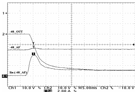
Figure 5. Input Voltage Turn-On Threshold CH1: -48_AF, CH2: -48V_OUT, CH4: lin(-48_AF)
