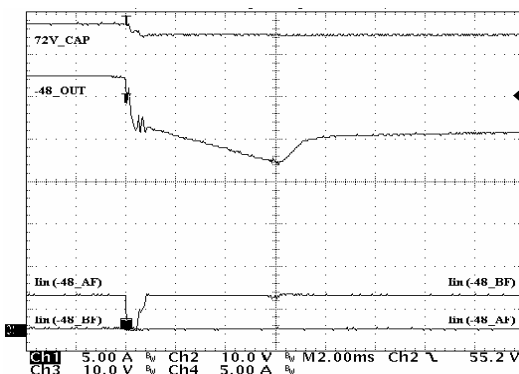
Figure 7. Loss of Feed A; Switchover to Feed B CH1: lin(-48_AF), CH2: -48V_OUT, CH3: lin(-48_BF), CH4: 72V_CAP
