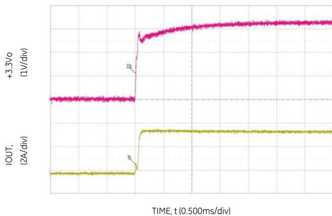
Fig 10: 3.3V Turn-On
