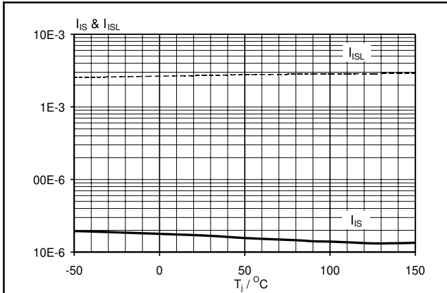
Fig. 14. Typical DC input currents. I_{IS} & I_{ISL} = f(T_j) ; normal & latched; conditions: V_{IS} = 5\text{ V} ; V_{PS} = 5\text{ V}
