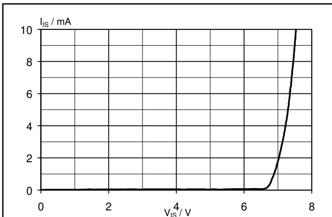
Fig. 16. Typical input clamping characteristic. I_I = f(V_{IS}) ; normal operation, T_j = 25^\circ\text{C}
