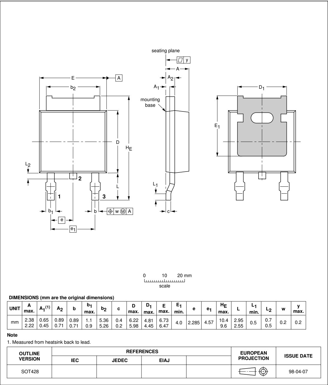
Fig.2. SOT428 surface mounting package 1 , centre pin connected to mounting base.
