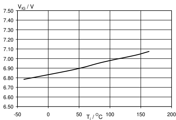
Fig. 18. Typical input clamping voltage. V_{IG} = f(T_j) ; condition I_L = 200\text{ }\mu\text{A} , V_{BG} = 13\text{ V}
