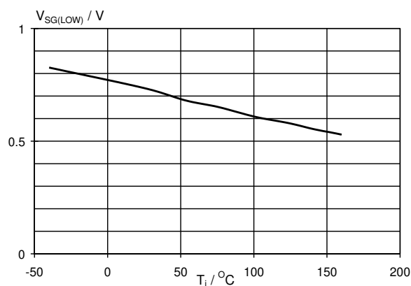
Fig. 16. Typical status low characteristic. V_{SG} = f(T_j) ; conditions V_{BG} \geq 9\text{ V} , I_S = 100\text{ }\mu\text{A}
