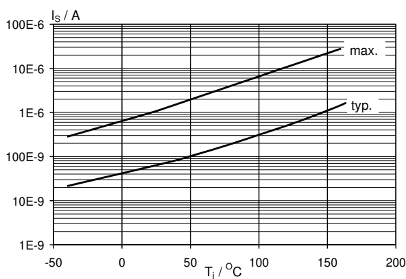
Fig. 12. Status leakage current. I_S = f(T_j) ; conditions V_{SG} = 5\text{ V} , V_{IG} = V_{BG} = 0\text{ V}
