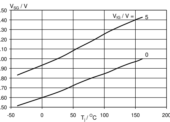
Fig. 20. Typical status clamping voltage. V_{SG} = f(T_j) ; condition I_S = 100\text{ }\mu\text{A} , V_{BG} = 13\text{ V}
