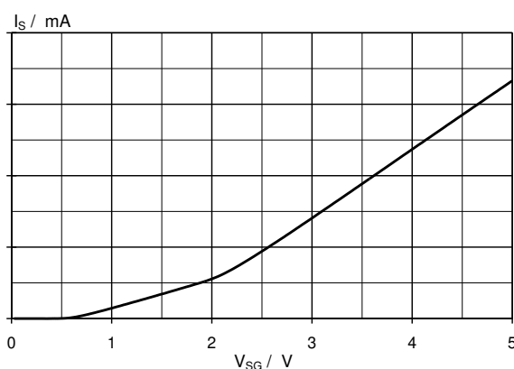
Fig. 19. Typical status low characteristic, T_j = 25\text{ }^\circ\text{C} . I_S = f(V_{SG}) ; conditions V_{IG} = 5\text{ V} , V_{BG} = 13\text{ V} , I_L = 0\text{ A}
