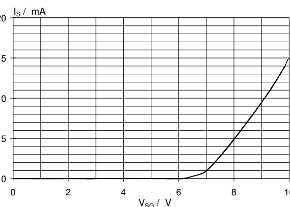
Fig. 21. Typical status characteristic, T_j = 25\text{ }^\circ\text{C} . I_S = f(V_{SG}) ; conditions V_{IG} = V_{BG} = 0\text{ V}
