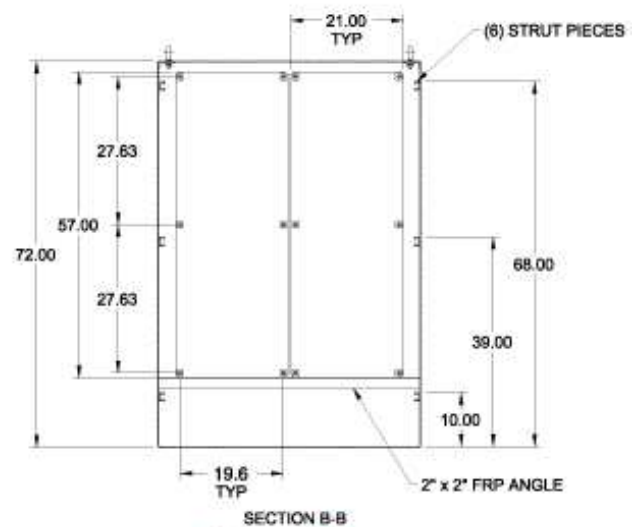
SECTION B-B Internal View
