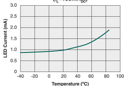
Typical I_F for Switch Operation vs. Temperature ( I_L = 100\text{mA}_{\text{DC}} )
