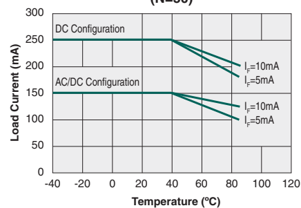
Maximum Load Current vs. Temperature (N=50)
