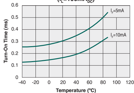
Typical Turn-On Time vs. Temperature ( I_L = 100\text{mA}_{\text{DC}} )
