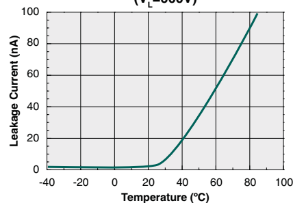
Typical Leakage vs. Temperature ( V_L=600\text{V} )
