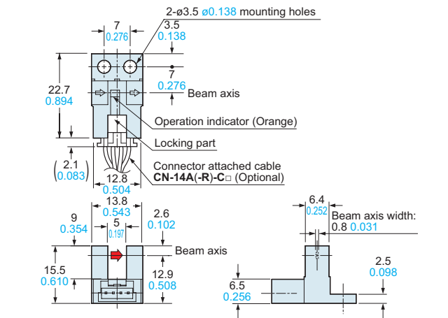
PM-Y64(P) Sensor
