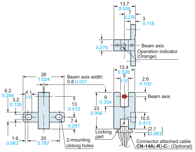
PM-L64(P) Sensor
