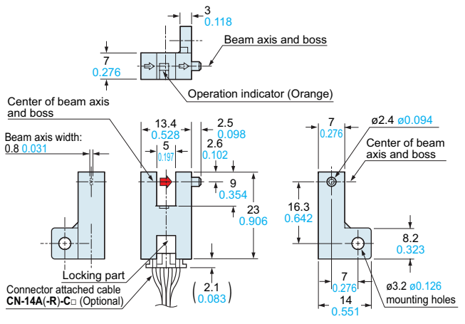
PM-F64(P) Sensor
