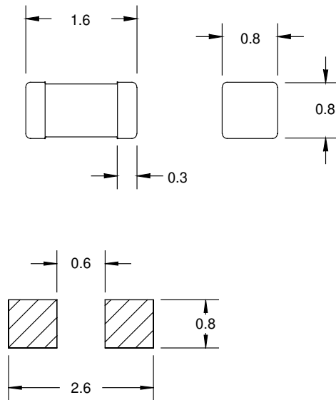
Pad Layout
