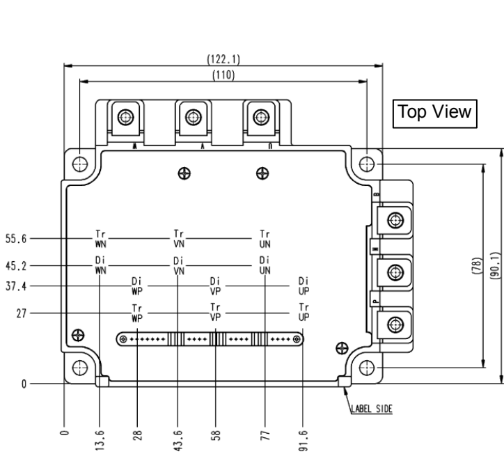
PM100CL1A120
