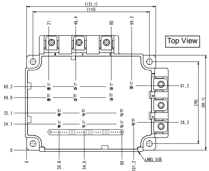
PM100RL1A120 350G
