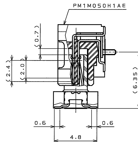
MATED CONDITION(REF.)
