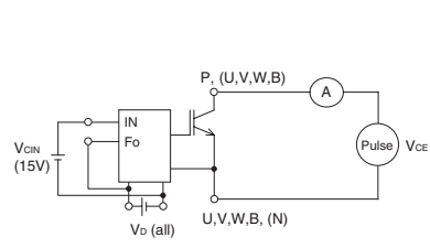
Fig. 3 Switching Time and SC Test Circuit
