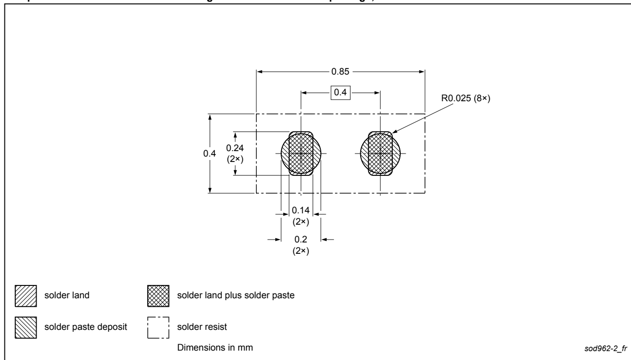
Fig. 16. Reflow soldering footprint for DSN0603-2 (SOD962-2)
