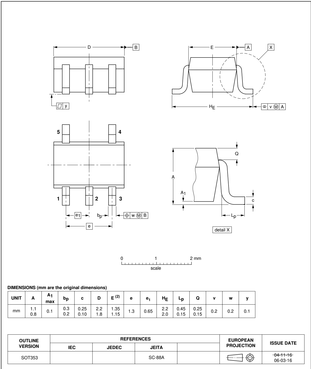
Fig 10. Package outline
