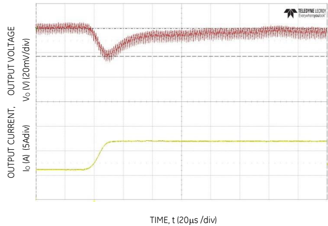
Figure 16. Transient Response to Dynamic Load Change from 50% to 100% at 12V in , C out =4x47uF+2x330uF, C Tune =8.2nF, R Tune =300
