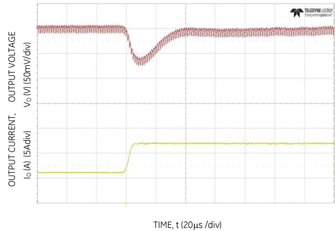
Figure 28 Transient Response to Dynamic Load Change from 50% to 100% at 12Vin, Cout=3x47µF+1x330µF, CTune=1800pF, RTune=300
