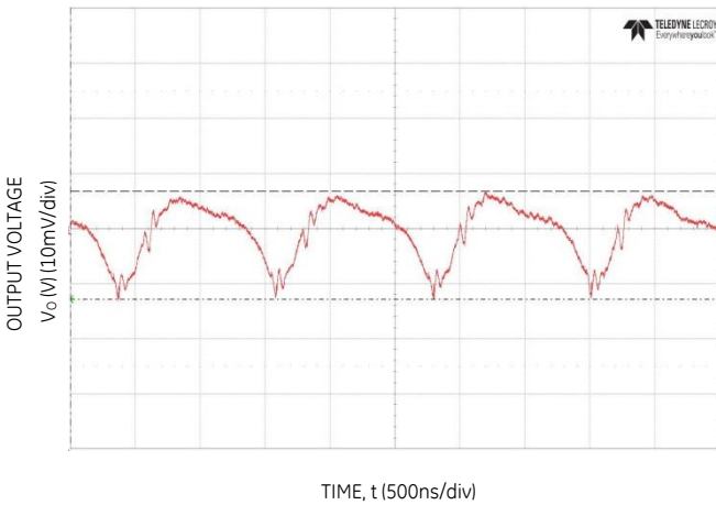
Figure 15. Typical output ripple (C o =2x47μF ceramic, V IN = 12V, I o = I o,max , 20MHz BW).
