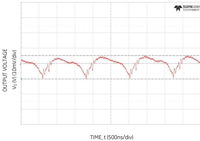
Figure 9. Typical output ripple (Co=2x47µF ceramic, VIN = 12V, Io = Io,max, 20MHz BW).
