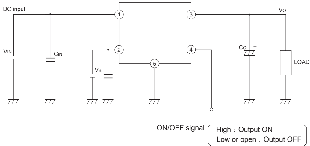
Fig.34 Typical Application
