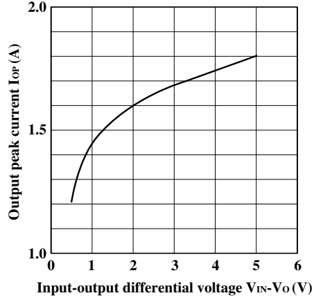
Fig.12 Output Peak Current vs. Input-output differential voltage
