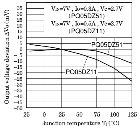
Fig.14 Output Voltage Deviation vs. Junction Temperature (PQ05DZ51/11)
