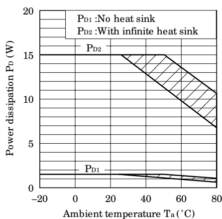
Fig. 4 Power Dissipation vs. Ambient Temperature (PQ15RW11/21)
