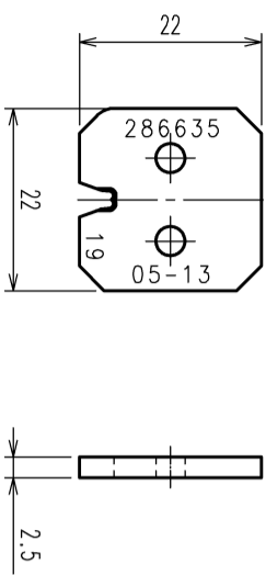
WIRE CRIMPER
