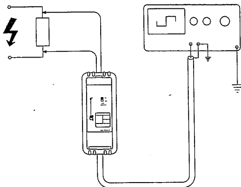
Differential probe for safe measurements
