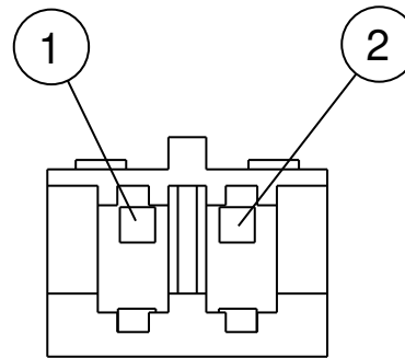
Connector B Manufacturer - JST Part #s PHR-2 Crimp Pin Part # SPH-002T-P0.5S Or equivalent Wire Entry View Scale 5.00
