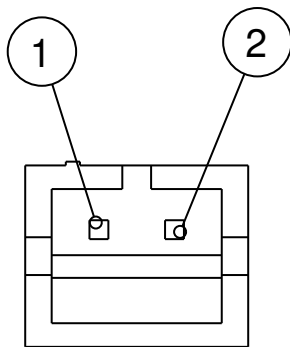
Connector A Manufacturer - JST Part #s S2B-PH-K-S Plug entry view
