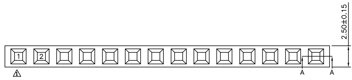
Recommended P.C.B Layout(Top Side) (PCB Board Tolerance \pm 0.05 )
