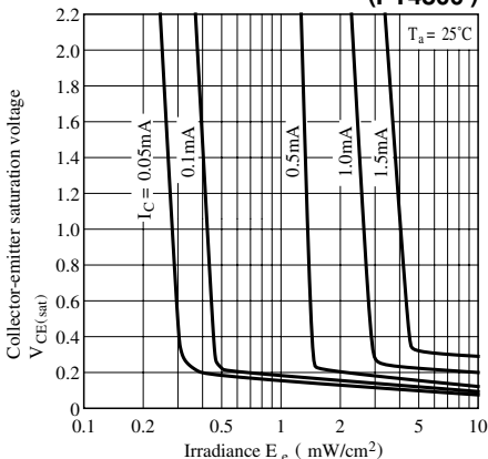
Fig. 9-a Collector-emitter Saturation Voltage vs. Irradiance (PT4800)
