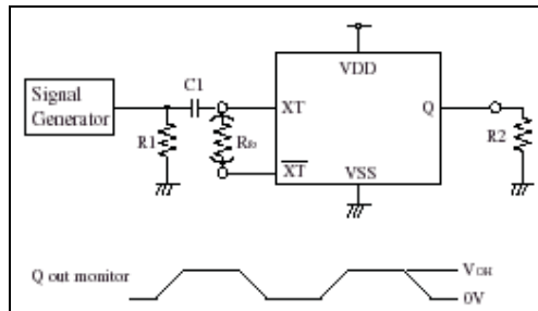
Measurement cct 1
