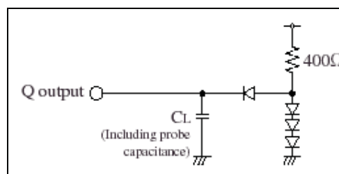
Load cct 2
