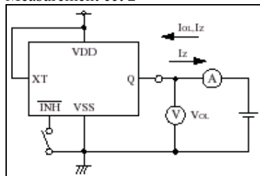
Measurement cct 2
