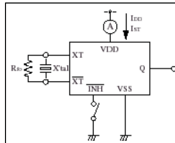
Measurement cct 3
