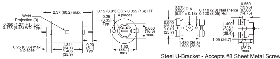
Steel U-Bracket - Accepts #8 Sheet Metal Screw
