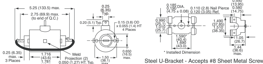
Steel U-Bracket - Accepts #8 Sheet Metal Screw
