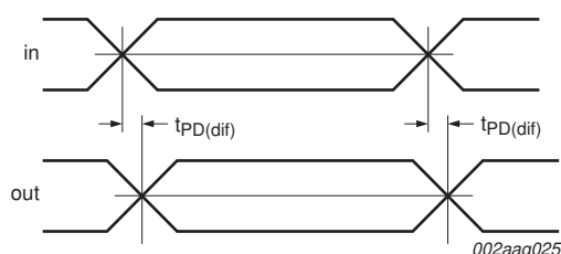
Fig 5. Propagation delay
