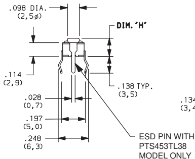
PTS453TL38 SPST
