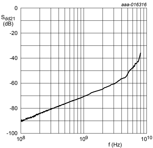
Sdd21 normalized to 100 Ω; differential pairs CH1/CH2 versus CH3/CH4 Fig. 3. Mixed-mode differential NEXT crosstalk; typical values
