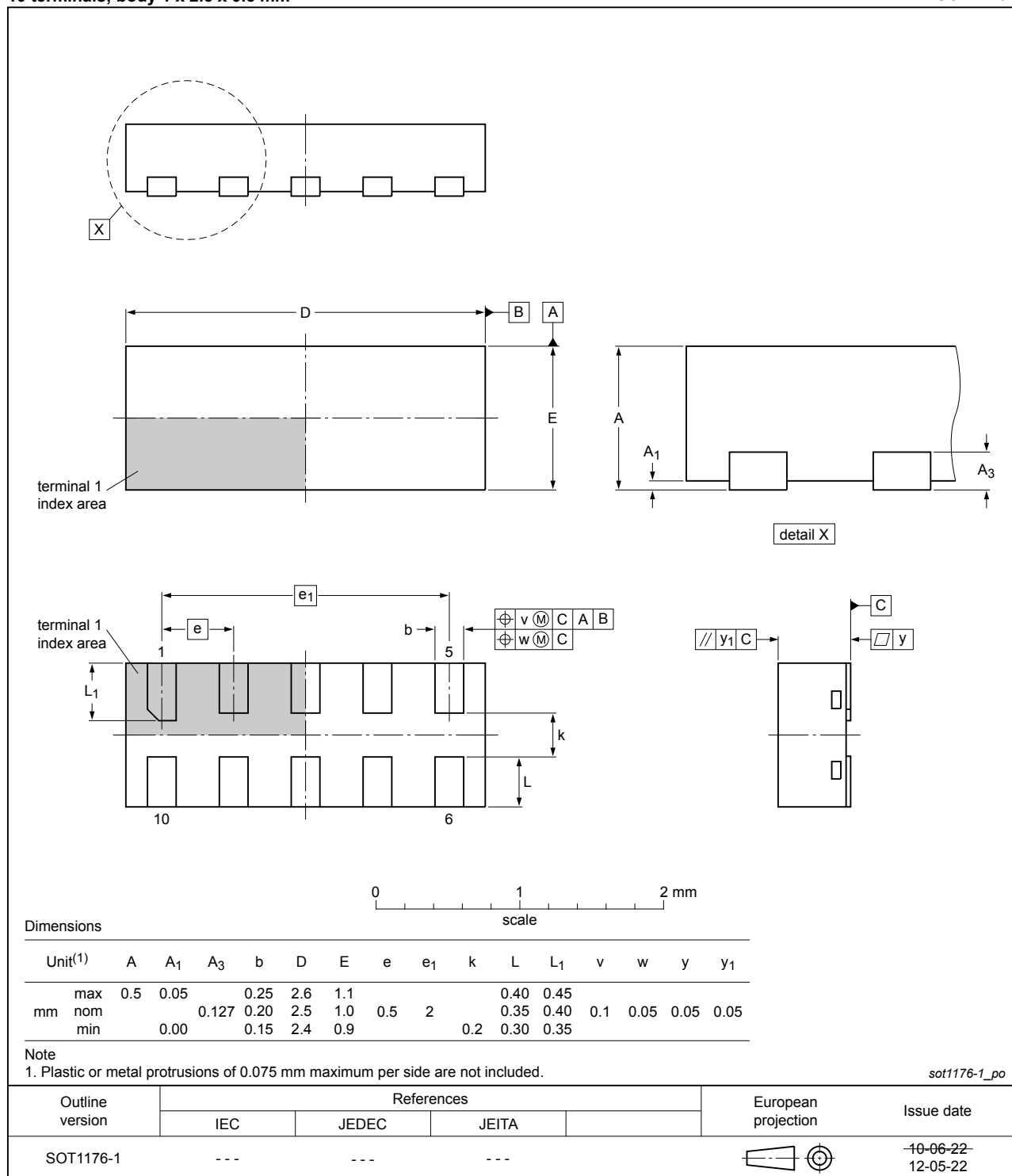
Fig. 13. Package outline DFN2510A-10 (SOT1176-1)
