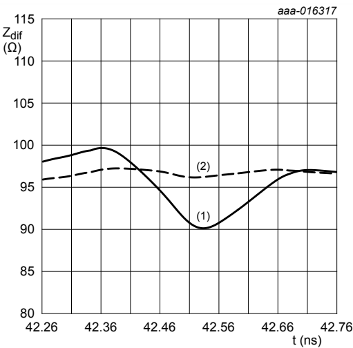
t_r = 200 \text{ ps} ; differential pair CH1 + CH2 (1) Device on reference board (2) Reference board without Device Under Test (DUT) Fig. 4. Differential Time Domain Reflectometer (TDR) plot; typical values
