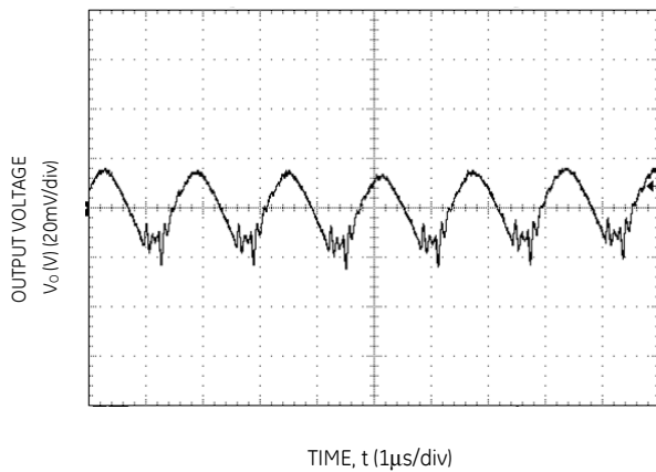
Figure 15. Typical output ripple and noise ( C_o=10\mu F ceramic, V_{IN} = 12V , I_o = I_{o,max} ).
