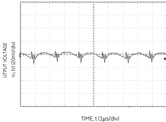
Figure 3. Typical output ripple and noise (C o =10μF ceramic, V IN = 8V, I o = I o,max ).
