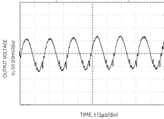
Figure 27. Typical output ripple and noise (C o =10μF ceramic, V IN = 12V, I o = I o,max ).
