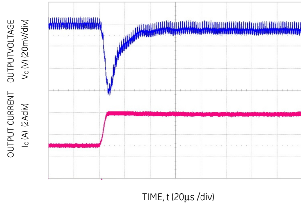
Figure 28. Transient Response to Dynamic Load Change from 50% to 100% at 12V in , C out -3x47μF, C Tune -178 & R Tune -3900pF
