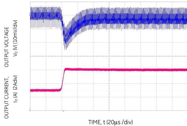
Figure 10. Transient Response to Dynamic Load Change from 50% to 100% at 12Vin, Cout-1x47uF+3x330uF, CTune-12nF & RTune-178
