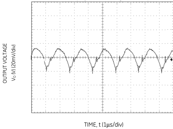
Figure 15. Typical output ripple and noise (Co=22μF ceramic, VIN = 12V, Io = Io,max.).
