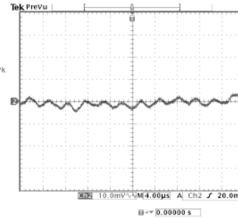
High Line, Full Load Ripple current= (9.2/10) \times 5=4.6\text{mA}
