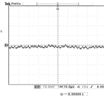
High Line, Full Load Ripple current= (6.2/10) \times 5=3.1\text{mA}
