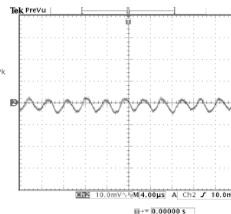
High Line, Full Load Ripple current= (8.6/10) \times 5=4.3\text{mA}
