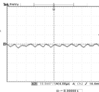
Normal Line, Full Load Ripple current= (6.6/10) \times 5=3.3\text{mA}
