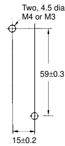
Mounting Holes
