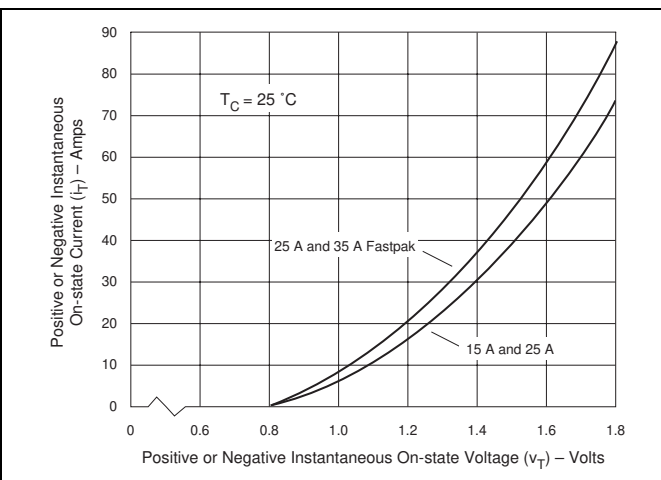
Figure E2.10 On-state Current versus On-state Voltage (Typical) (15 A and 25 A)
