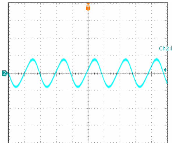
Figure 15: Output voltage ripple at nominal input voltage and rated load current ( I_o=33\text{A} ) (50 mV/div, 2 \mu\text{s} /div) Load capacitance: 1\mu\text{F} ceramic capacitor and 10\mu\text{F} tantalum capacitor. Bandwidth: 20 MHz. Scope measurements should be made using a BNC cable (length shorter than 20 inches). Position the load between 51 mm to 76 mm (2 inches to 3 inches) from the module.
