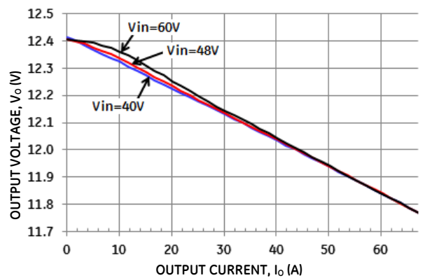
Figure 12. Typical Output Voltage Regulation vs. Output Current with the -P option.
