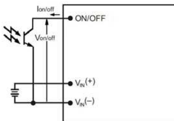
Figure 16. Remote On/Off Implementation.
