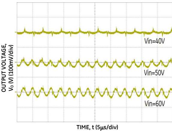
Figure 3. Typical Output Ripple and Noise, I_o = I_{o,max} , C_o = 750\mu F .
