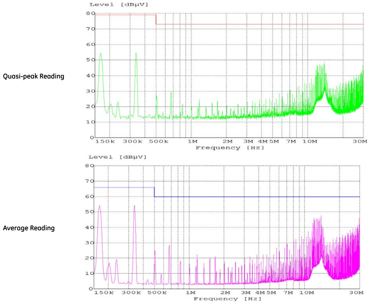
Figure 26. EMC Consideration
