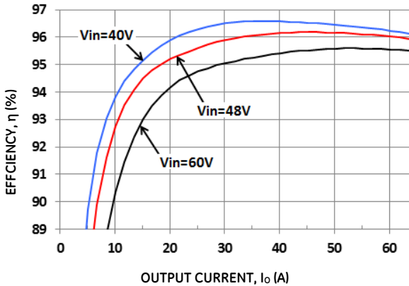
Figure 1. Typical Converter Efficiency vs. Output Current.
